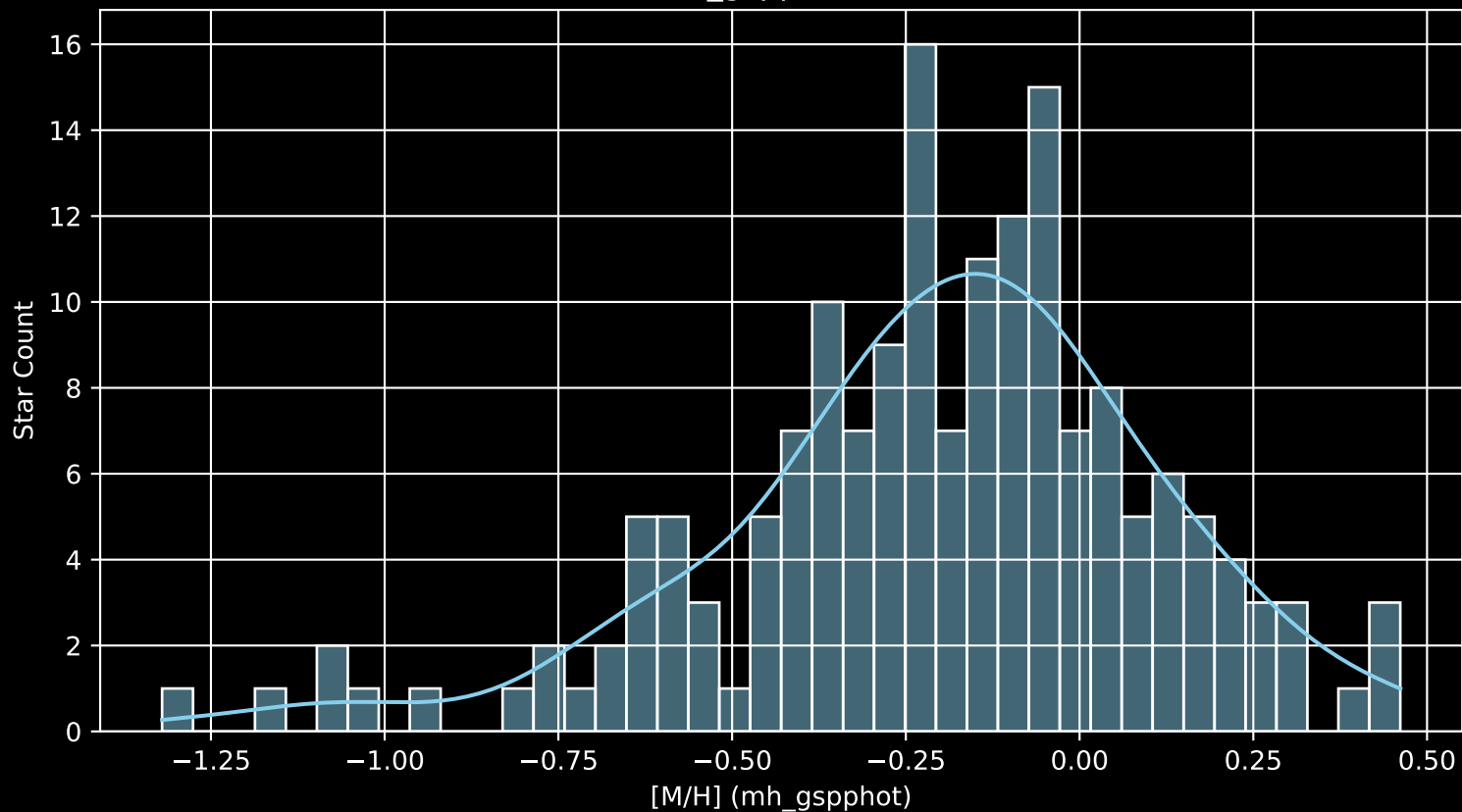
APOGEE DR17 Field: [081+34_MGA [M/H] (mh_gspphot) (n= 170)
