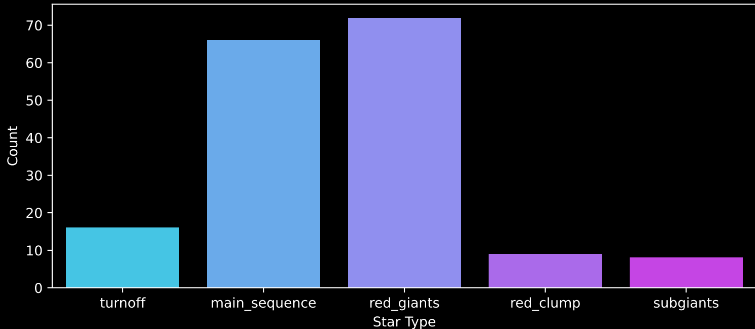
APOGEE DR17 Field: [081+34_MGA] Count plot of Star Type
