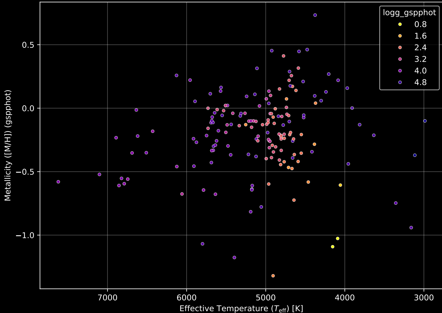
APOGEE DR17 Field: [081+34_MGA] Stellar Population Parameters (n= 171)
