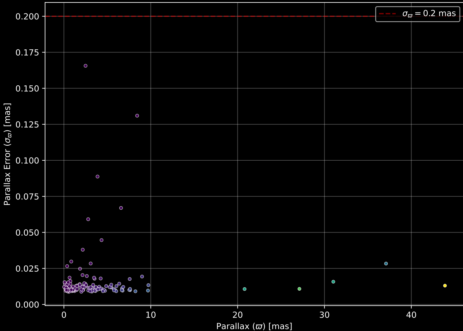
APOGEE DR17 Field: [081+34_MGA] Parallax Quality (n= 171)
