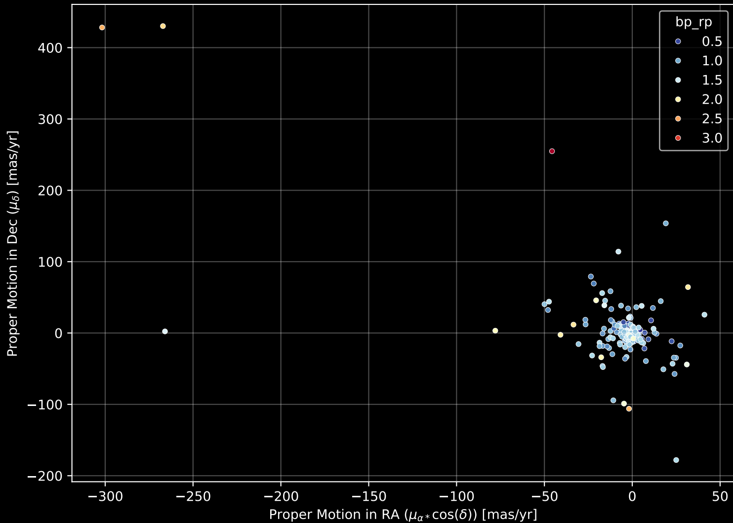
APOGEE DR17 Field: [081+34_MGA] Proper Motion Diagram (n= 171)
