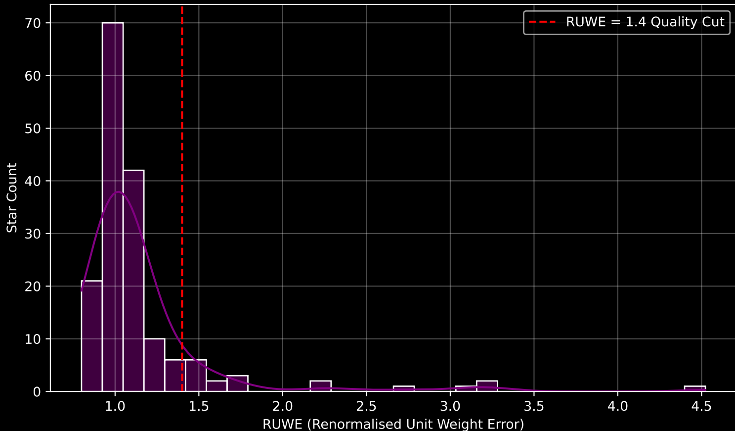
GAPOGEE DR17 Field [081+34_MGA] RUWE Distribution (n= 167)
